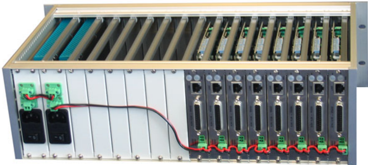
Rear view of the UCF-16.3
